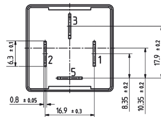
View of the Terminals (bottom view)
