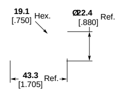
N Series Plug to 7 mm Best VSWR Jack
