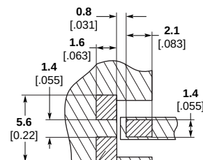
Ground Pad Typ. Signal Pad Recommended Mounting Pattern
