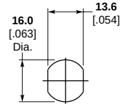
Recommended Mounting Hole
