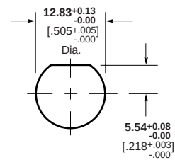
Maximum Panel Thickness 6.1 [.240] Recommended Panel Cutout
