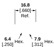
MCX Jack – SMA Plug
