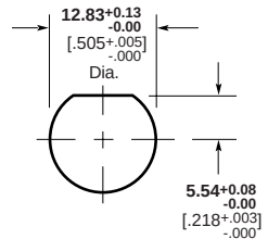
Maximum Panel Thickness 6.1 [.240] Recommended Panel Cutout
