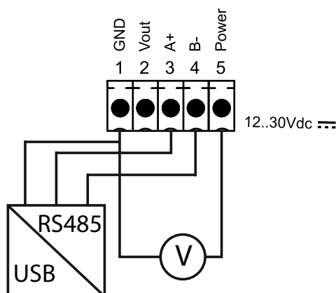
Connection scheme BT7100
