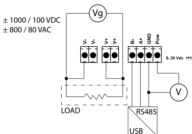
Connection scheme BT7200 / BT7250
