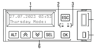
Abb. 12 Frontplatte
