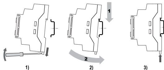
Abb. 2 Installation
