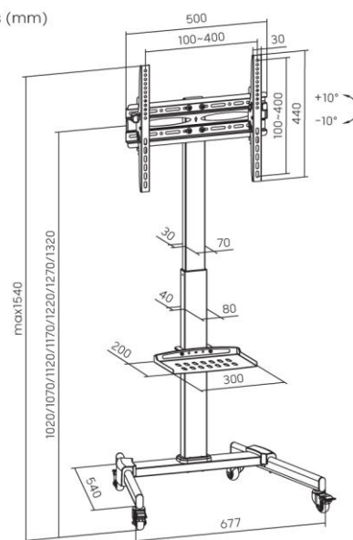
Dimensions (mm)
