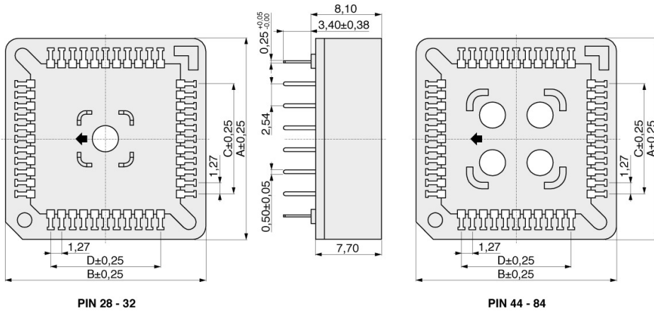
PIN 28 - 32
