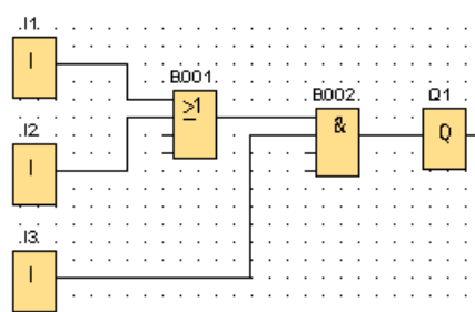
Stromlaufplan in LOGO!Soft Comfort
