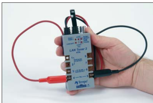
Check to see if a jack has telephone service.
