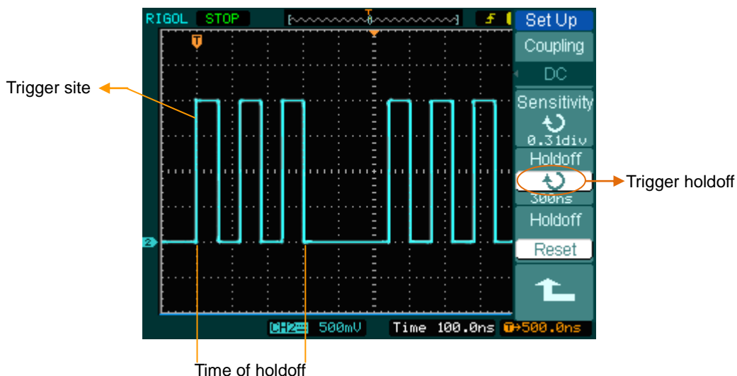
Figure 2- 65 Trigger Holdoff
