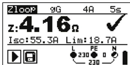
Figure 5.25: Examples of loop impedance measurement result
