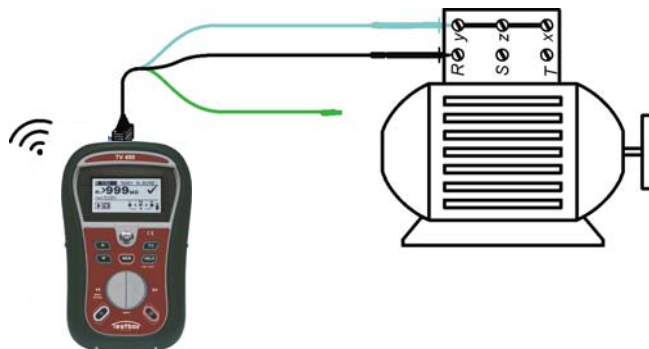
Figure 5.11: 3-wire test lead application
