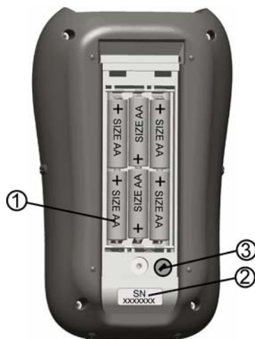
Figure 3.4: Battery compartment
