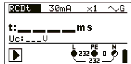
Figure 5.16: RCD test
