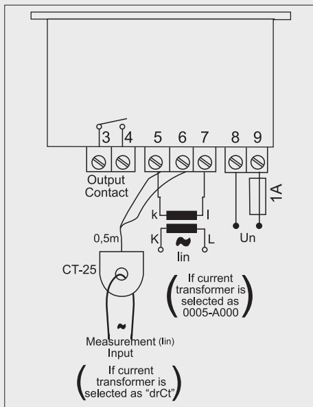
EPM-4C PR20 (48x96)
