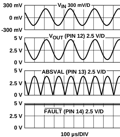
Figure 19. Sine response 400 mV pk to pk 4 kHz input, at V_{\text{REF}} = 5 \text{ V} .
