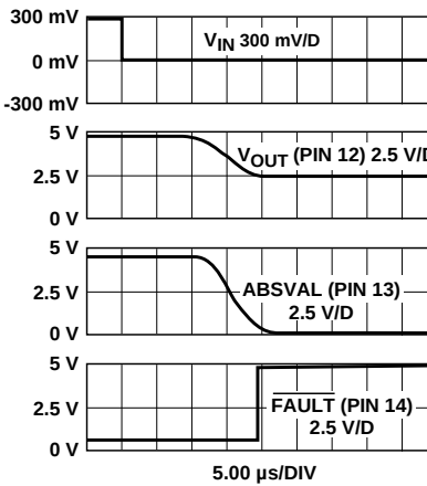
Figure 16. \overline{\text{FAULT}} release, 300 to 0 mV input, at V_{\text{REF}} = 5 \text{ V} .
