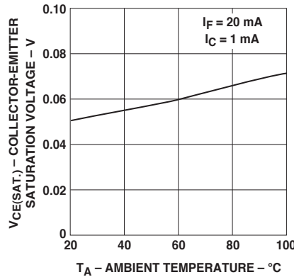
Figure 8. Collector-emitter saturation voltage vs. temperature.
