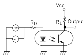
Test Circuit for Frequency Response
