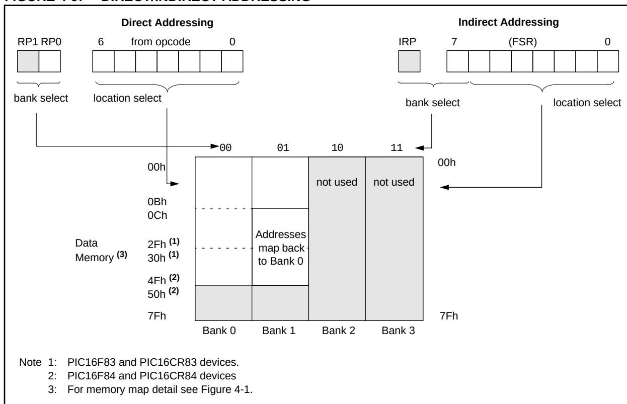
FIGURE 4-9: DIRECT/INDIRECT ADDRESSING
