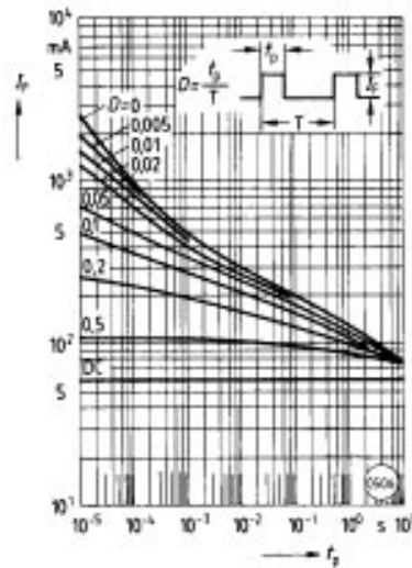
Figure 5. Permissible pulse handling capability. Forward current vs. pulse width Pulse cycle D=\text{parameter} , T_A=25^\circ\text{C}
