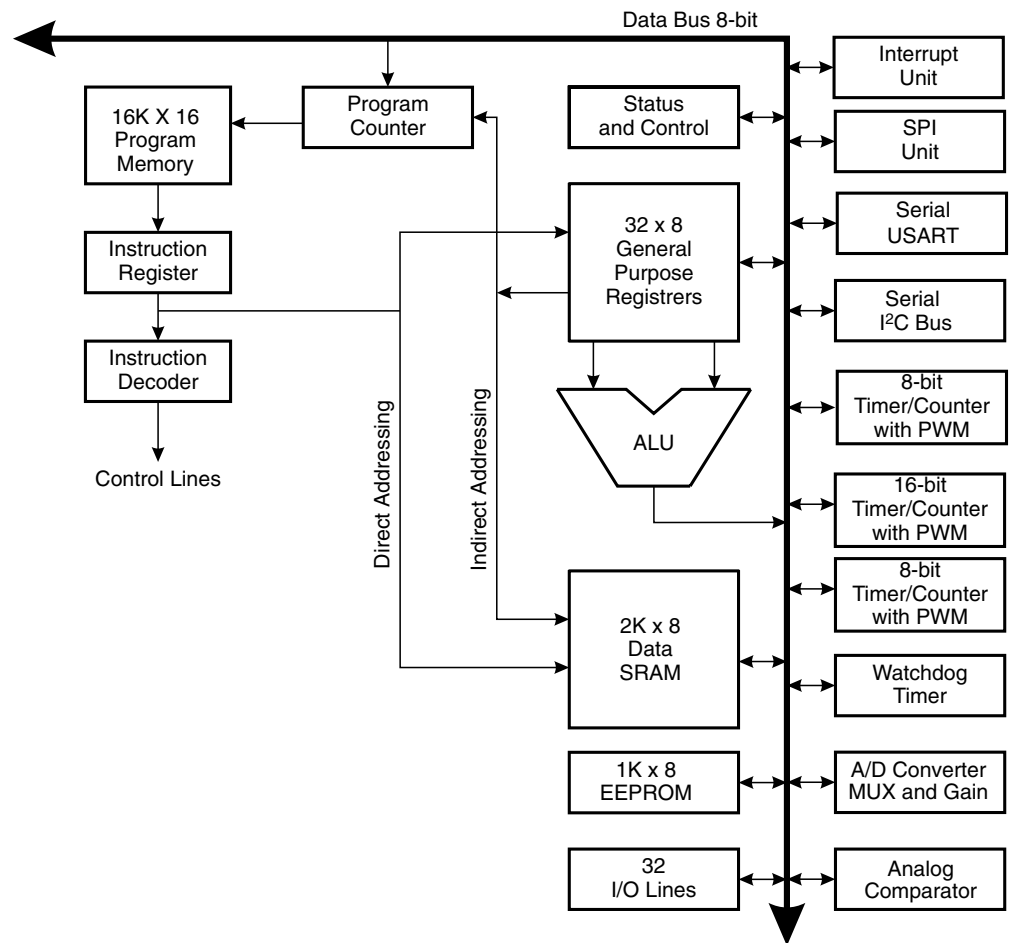
Figure 5. The ATmega323 AVR Enhanced RISC Architecture
