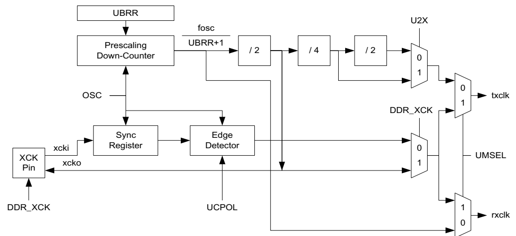
Figure 46. Clock Generation Logic, Block Diagram
