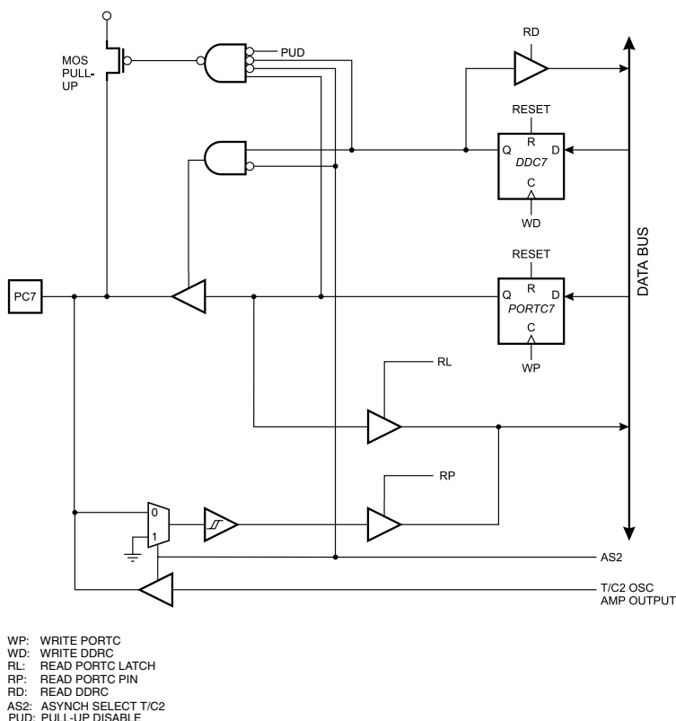
Figure 78. Port C Schematic Diagram (Pins PC7)
