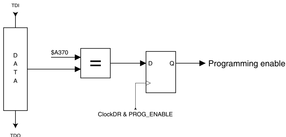
Figure 101. Programming Enable Register
