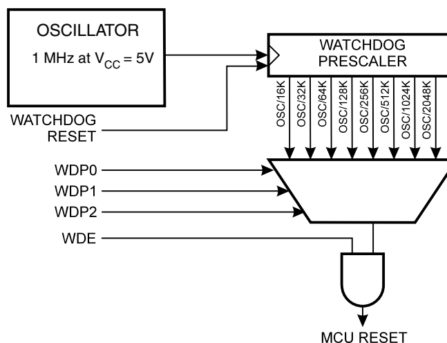
Figure 40. Watchdog Timer
