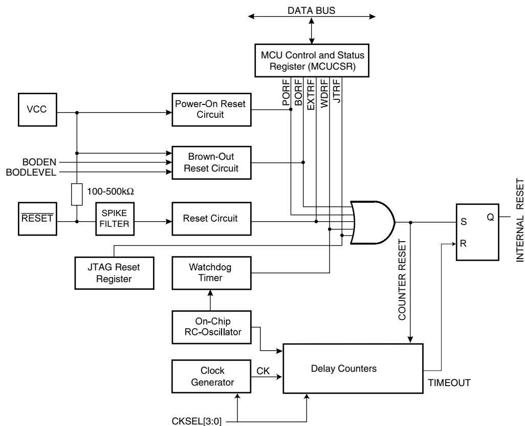
Figure 24. Reset Logic
