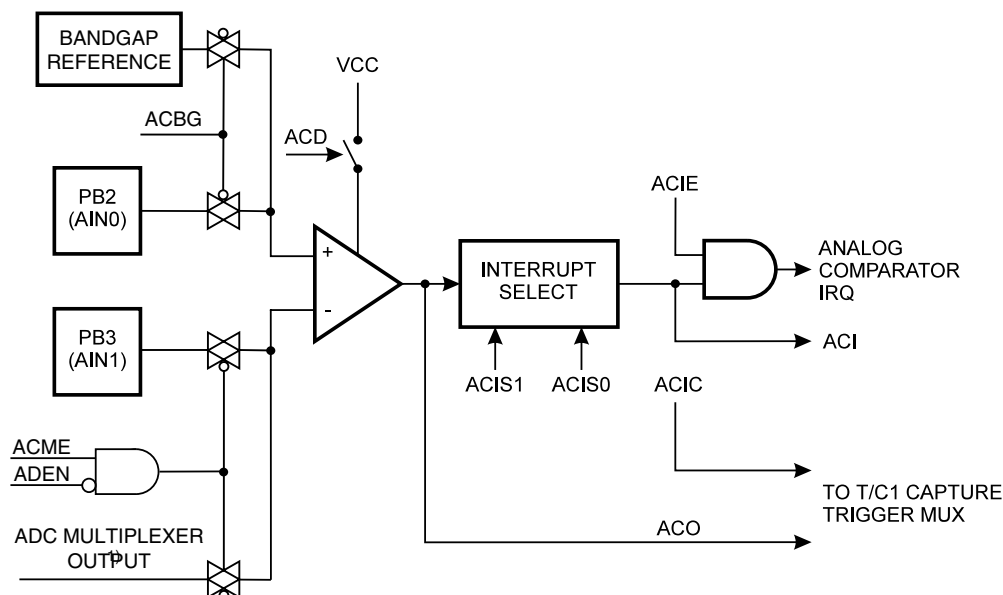
Figure 59. Analog Comparator Block Diagram
