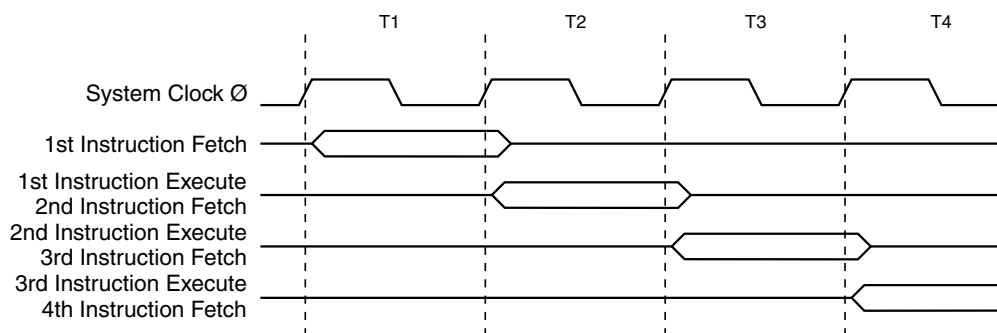
Figure 21. The Parallel Instruction Fetches and Instruction Executions
