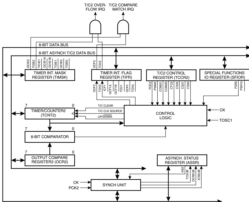
Figure 33. Timer/Counter2 Block Diagram
