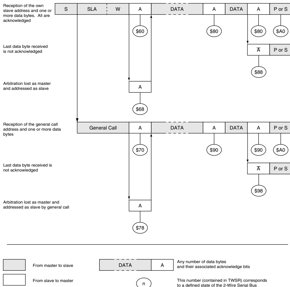
Figure 57. Formats and States in the Slave Receiver Mode
