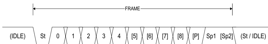
Figure 48. Frame Formats
