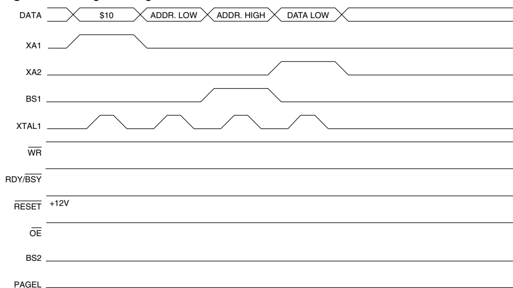
Figure 94. Programming the Flash Waveforms
