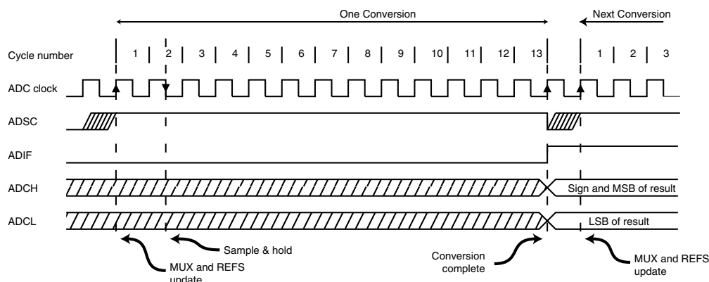
Figure 63. ADC Timing Diagram, Single Conversion
