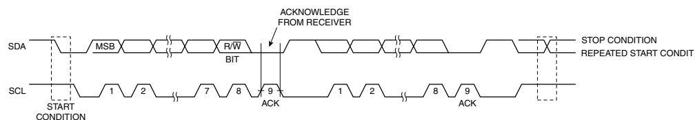
Figure 53. 2-wire Serial Bus Timing Diagram
