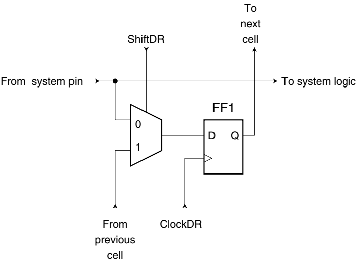
Figure 91. Observe-only Cell
