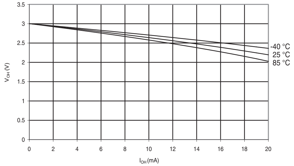
Figure 28-268. ATmega644PA: I/O Pin Output Voltage vs. Source Current ( V_{CC} = 3V ).
