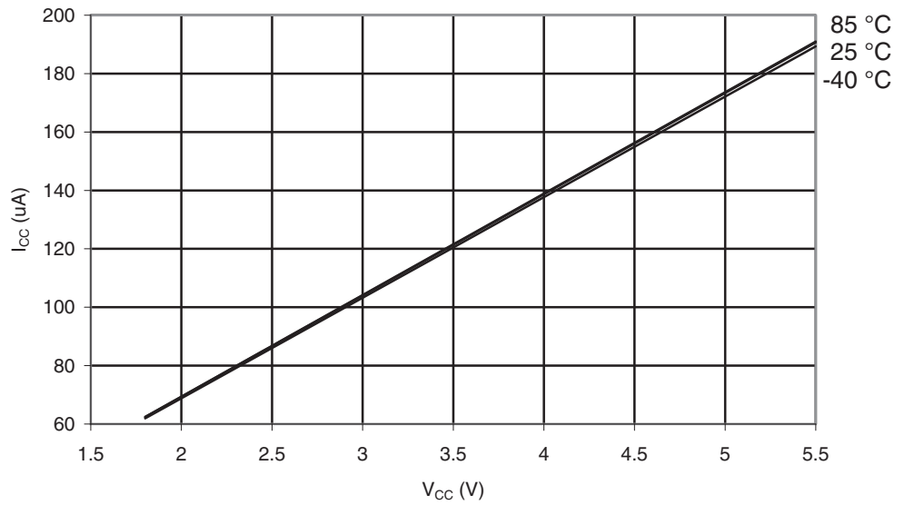
Figure 28-388. ATmega1284P: AREF External Reference Current vs. V_{CC}
