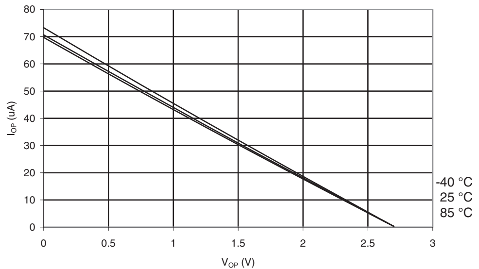
Figure 28-310. ATmega1284: I/O Pin Pull-up Resistor Current vs. Input Voltage ( V_{CC} = 2.7V )
