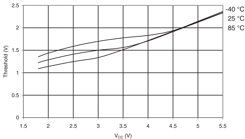
Figure 28-28. ATmega164A: Reset Pin Input Threshold vs. V_{CC} ( V_{IH} , I/O Pin Read as '1').
