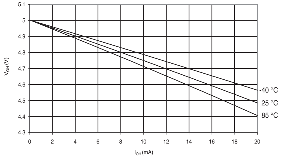
Figure 28-269. ATmega644PA: I/O Pin Output Voltage vs. Source Current ( V_{CC} = 5V ).
