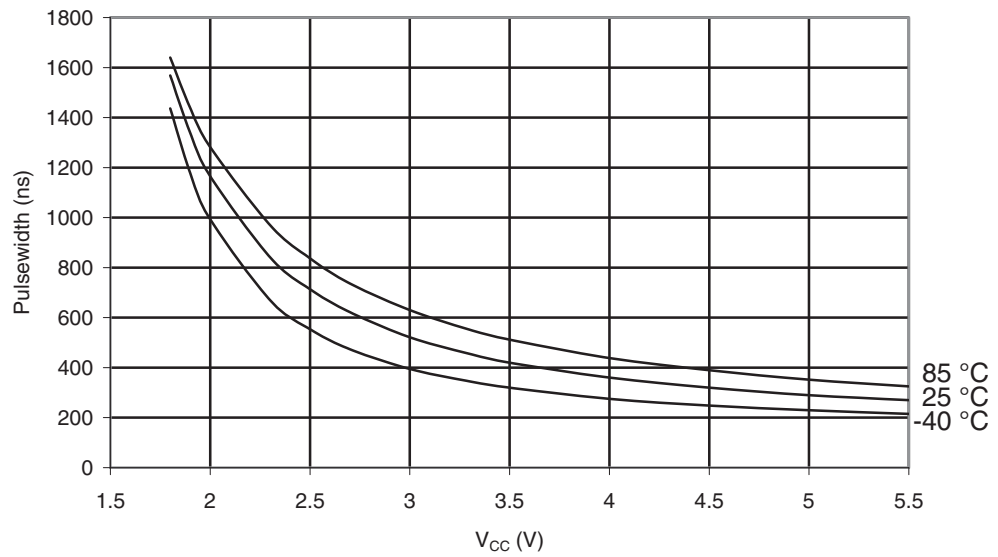
Figure 28-394. ATmega1284P: Minimum Reset Pulsethwidth vs. V_{CC}
