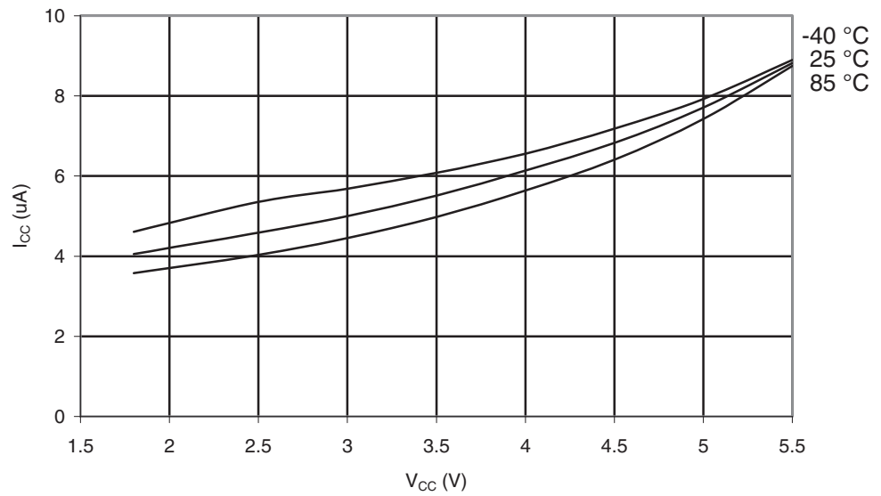
Figure 28-61. ATmega164PA: Power-down Supply Current vs. V_{CC} (Watchdog Timer Enabled).
