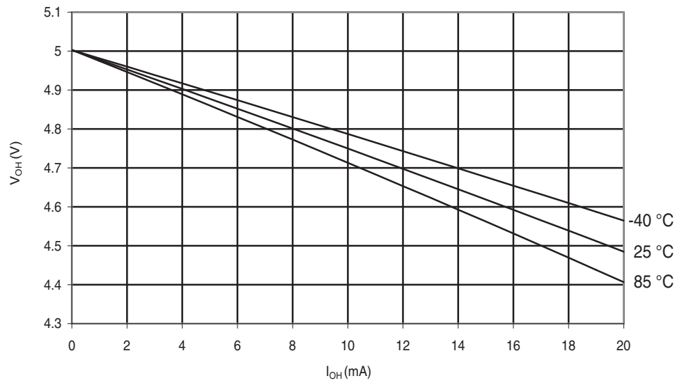
Figure 28-220. ATmega644A: I/O Pin Output Voltage vs. Source Current ( V_{CC} = 5V )
