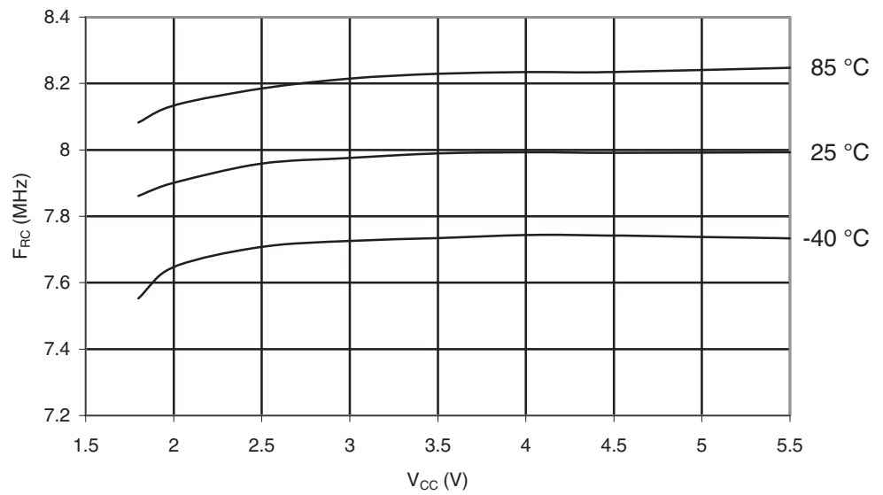
Figure 28-87. ATmega164PA: Calibrated 8 MHz RC Oscillator vs. V_{CC}
