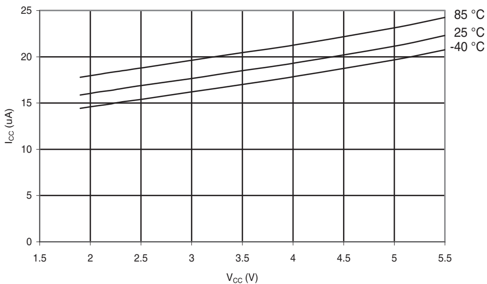
Figure 28-142. ATmega324A: Brownout Detector Current vs. V_{CC}
