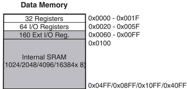
Figure 7-2. Data Memory Map for ATmega164A/164PA/324A/324PA/644A/644PA/1284/1284P
