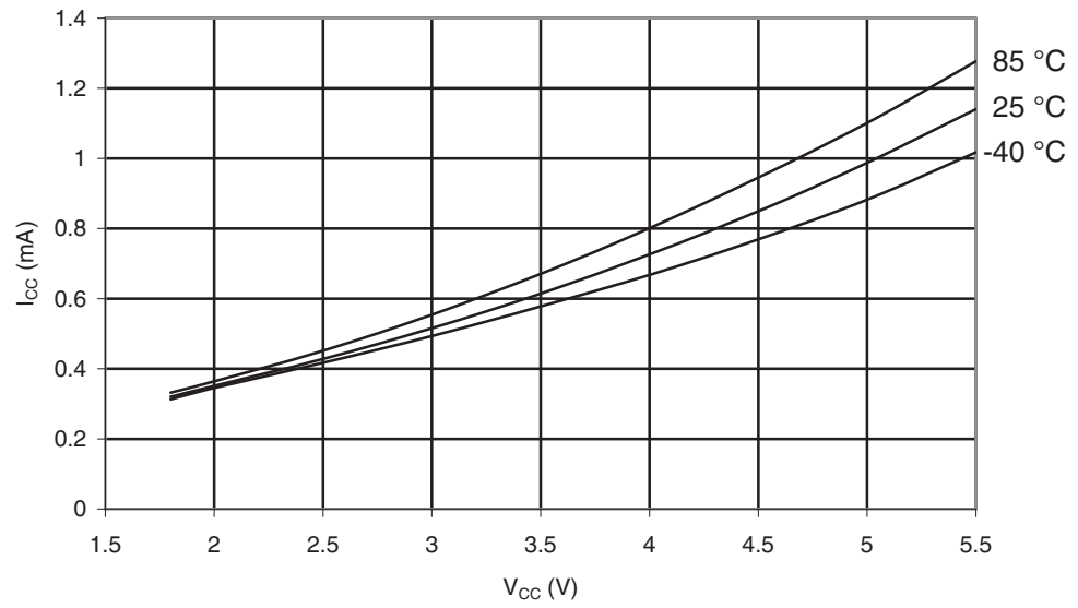
Figure 28-302. ATmega1284: Idle Supply Current vs. V_{CC} (Internal RC Oscillator, 8 MHz)
