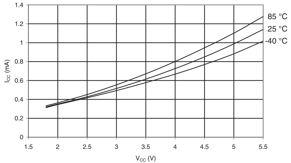
Figure 28-352. ATmega1284P: Idle Supply Current vs. V_{CC} (Internal RC Oscillator, 8 MHz)
