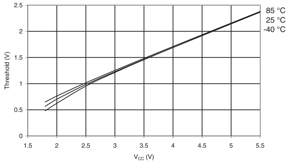
Figure 28-26. ATmega164A: I/O Pin Input Threshold vs. V_{CC} ( V_{IL} , I/O Pin Read as '0').
