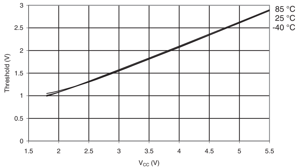
Figure 28-74. ATmega164PA: I/O Pin Input Threshold vs. V_{CC} ( V_{IH} , I/O Pin Read as '1').
