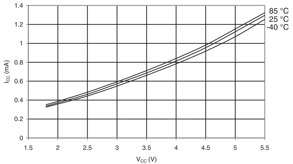
Figure 28-200. ATmega644A: Active Supply Current vs. V_{CC} (Internal RC Oscillator, 1 MHz).
