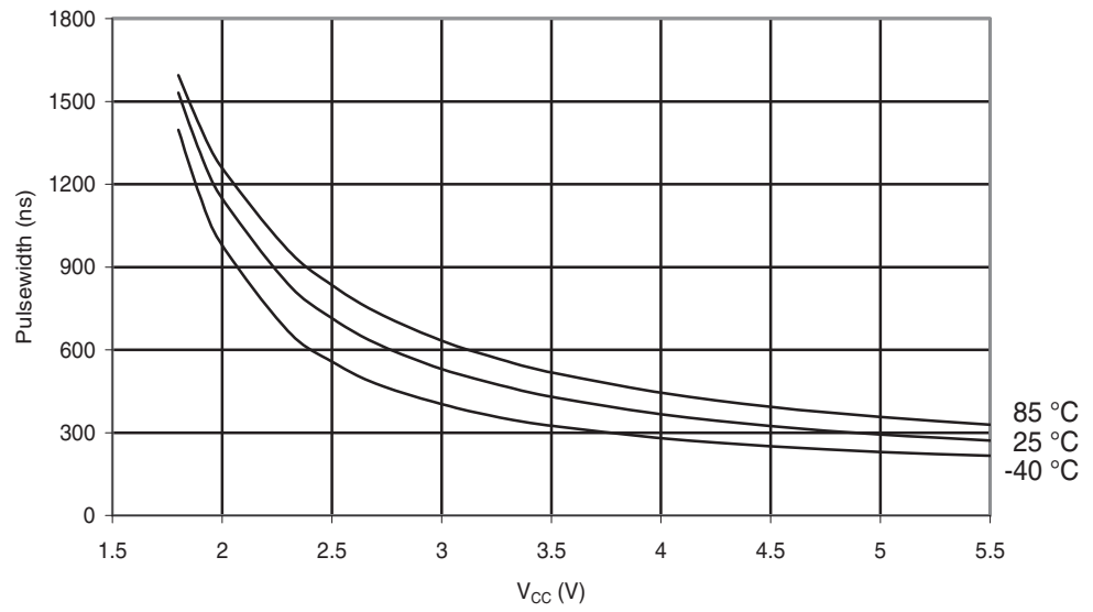
Figure 28-196. ATmega324PA: Minimum Reset Pulsewidth vs. V_{CC}
