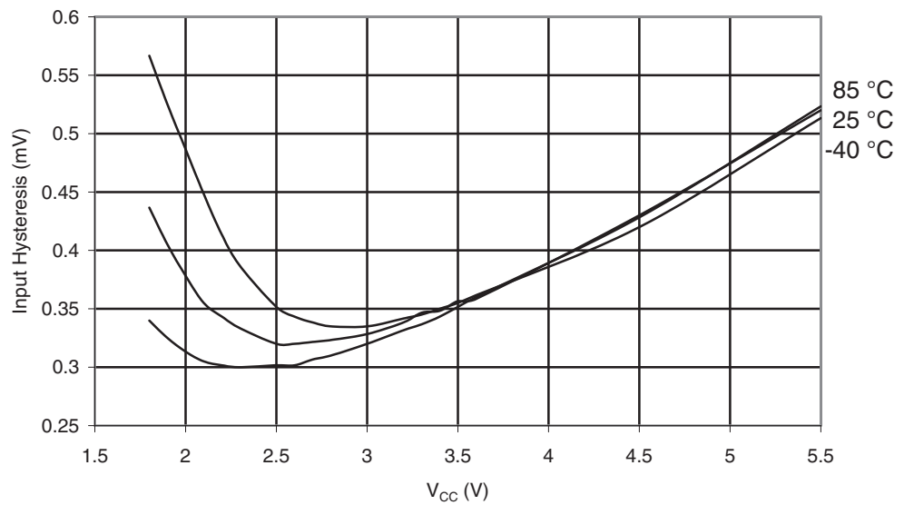
Figure 28-322. ATmega1284: I/O Pin Input Hysteresis vs. V_{CC}
