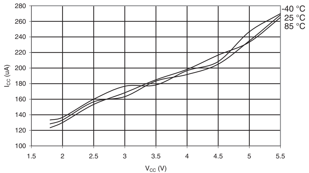
Figure 28-386. ATmega1284P: ADC Current vs. V_{CC} (AREF = AV_{CC} )
