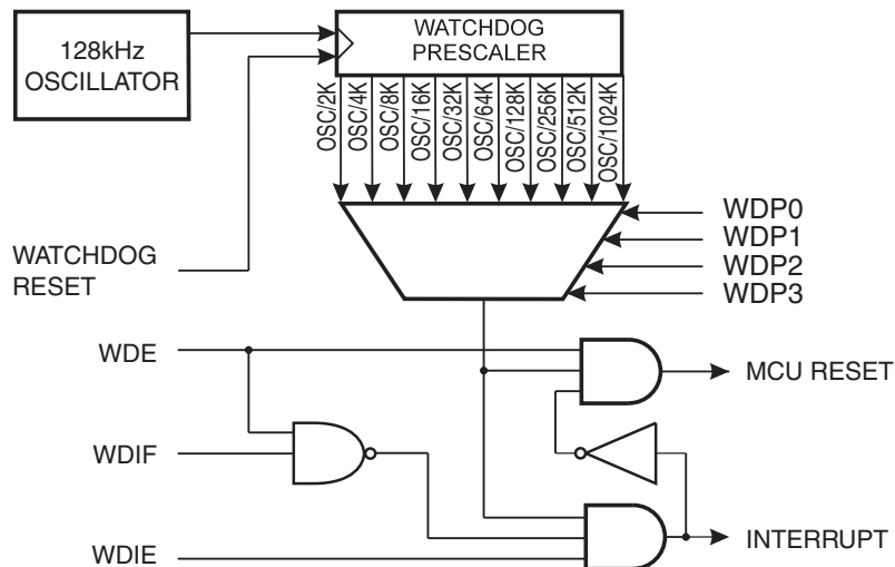
Figure 10-7. Watchdog Timer
