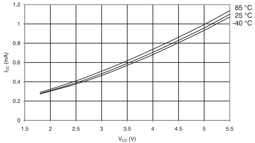
Figure 28-8. ATmega164A: Idle Supply Current vs. V_{CC} (Internal RC Oscillator, 8 MHz).
