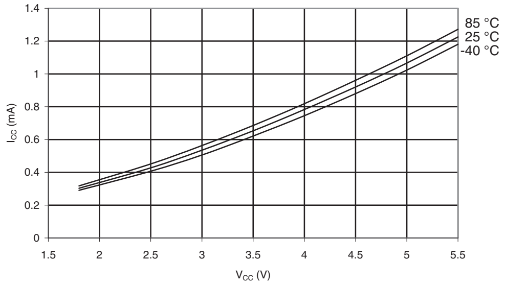
Figure 28-204. ATmega644A: Idle Supply Current vs. V_{CC} (Internal RC Oscillator, 8 MHz).
