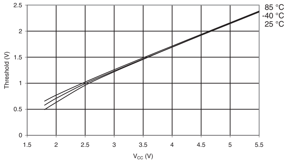
Figure 28-321. ATmega1284: I/O Pin Input Threshold vs. V_{CC} ( V_{IL} , I/O Pin Read as '0')
