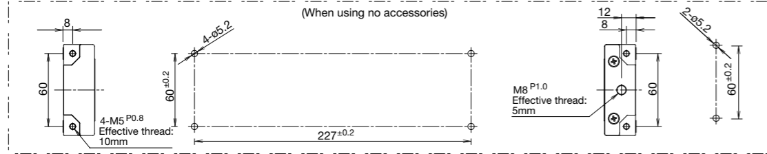
Mounting Hole Layout
