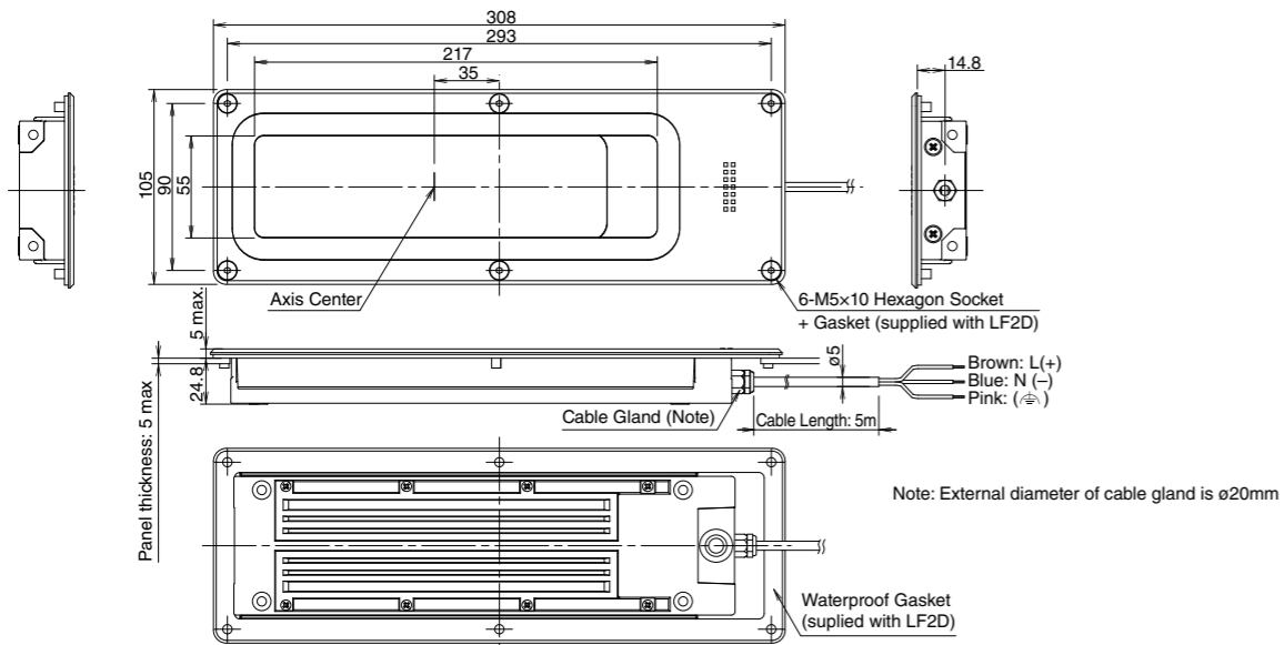
Mounting Hole Layout
