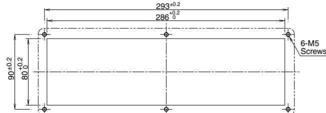
Mounting Hole Layout
