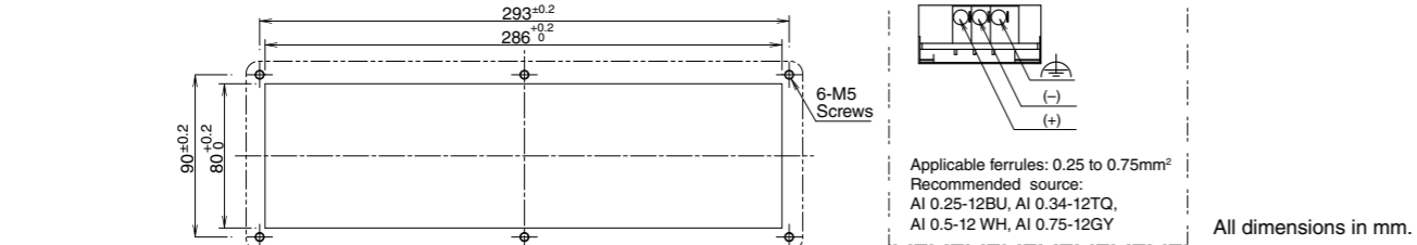
Mounting Hole Layout
