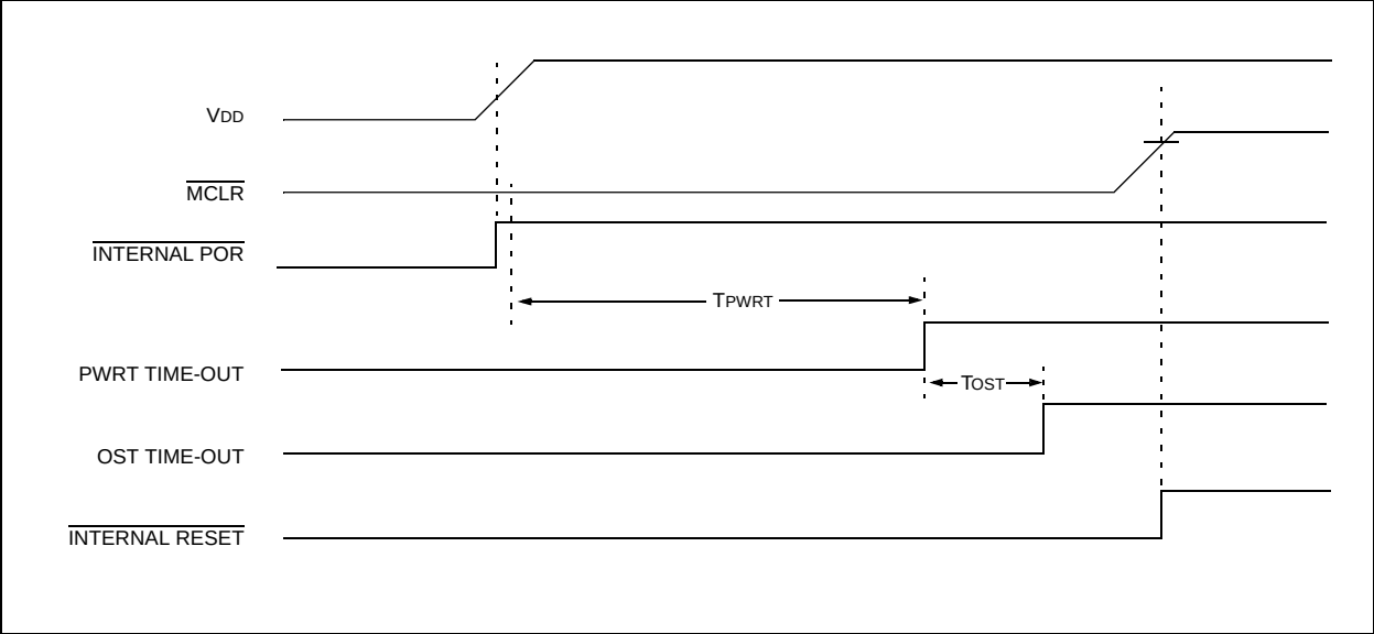
FIGURE 11-7: TIME-OUT SEQUENCE ON POWER-UP (MCLR NOT TIED TO VDD): CASE 2
