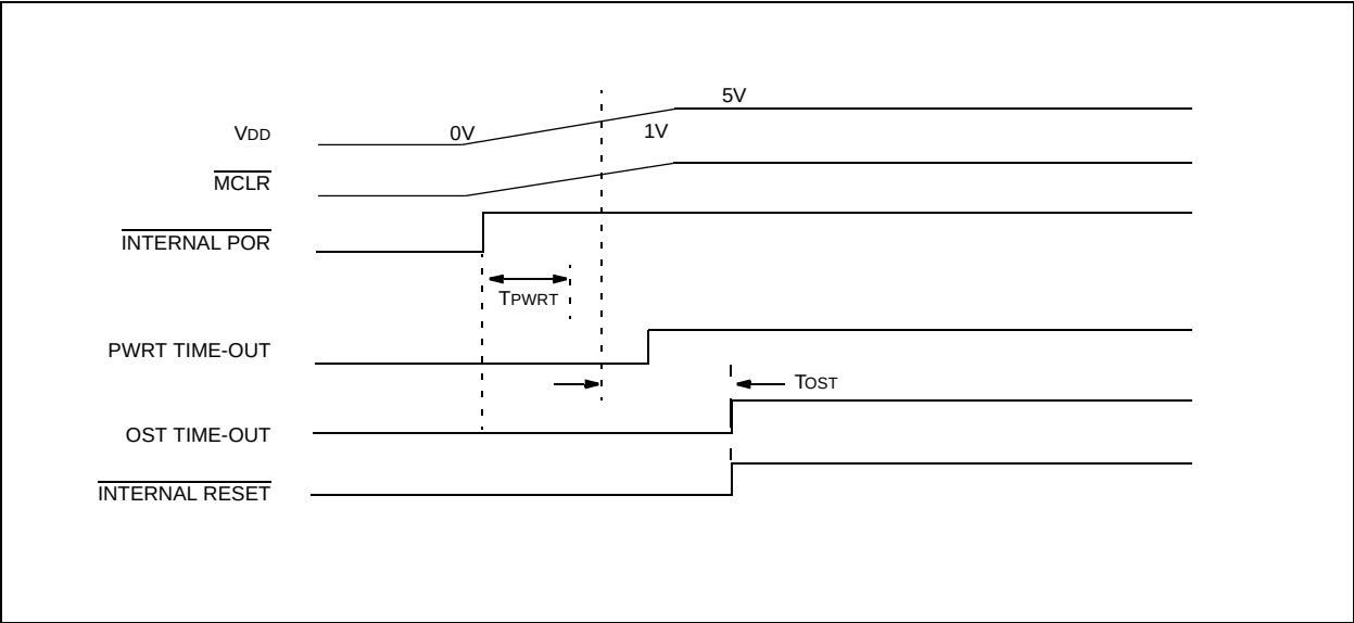
FIGURE 11-8: SLOW RISETIME (MCLR TIED TO VDD VIA RC NETWORK)
