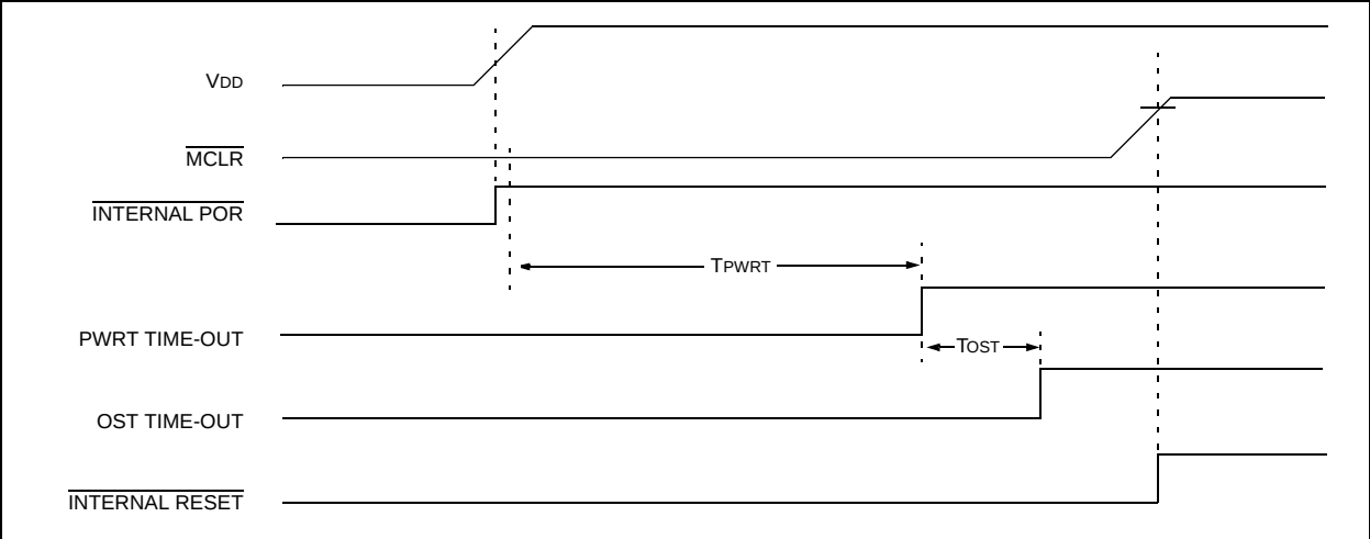
FIGURE 12-8: TIME-OUT SEQUENCE ON POWER-UP (MCLR NOT TIED TO VDD): CASE 2
