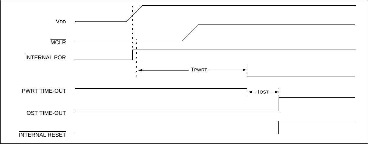
FIGURE 12-7: TIME-OUT SEQUENCE ON POWER-UP (MCLR NOT TIED TO VDD): CASE 1
