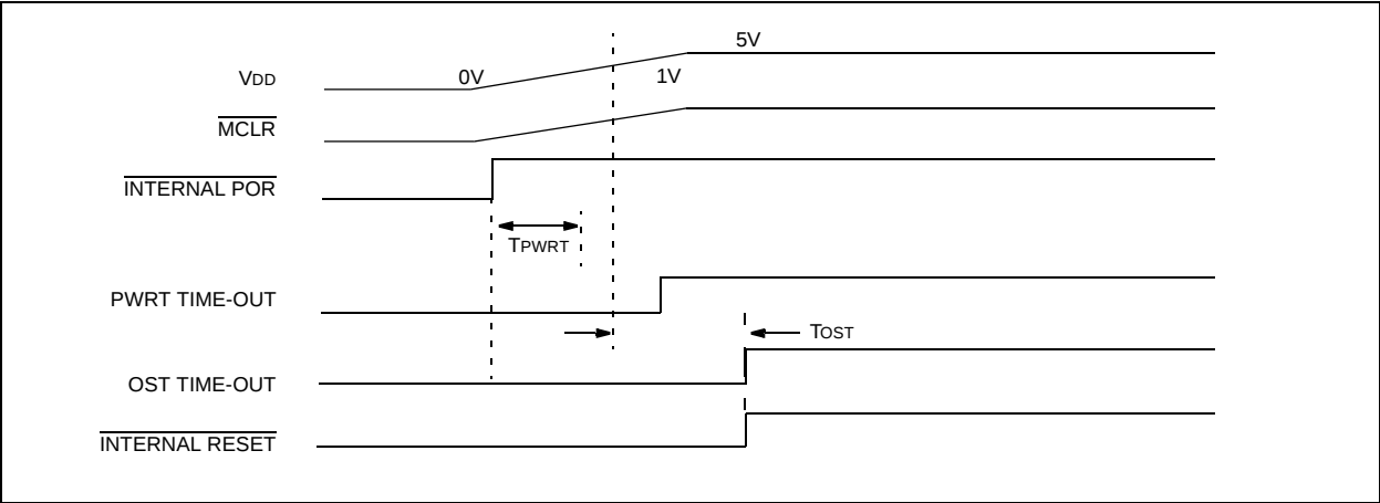
FIGURE 12-9: SLOW RISE TIME (MCLR TIED TO VDD THROUGH RC NETWORK)
