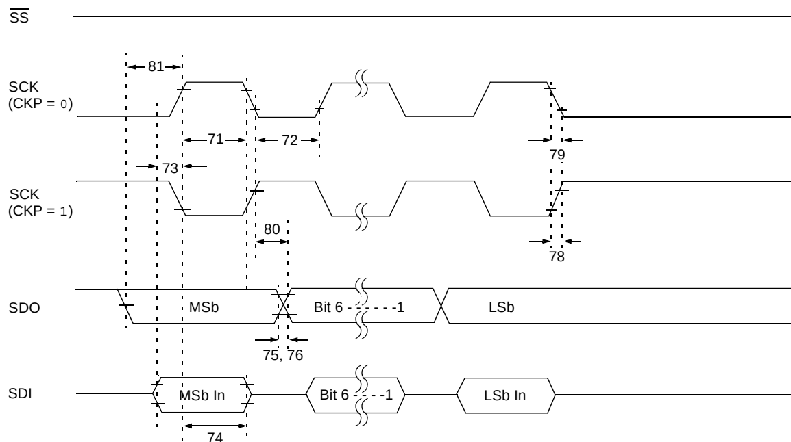
FIGURE 15-11: SPI™ MASTER MODE TIMING (CKE = 1, SMP = 1)
