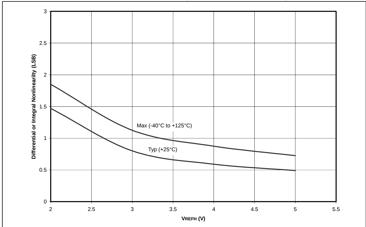
FIGURE 19-26: A/D NONLINEARITY vs. VREFH (VDD = 5V, -40°C TO +125°C)
