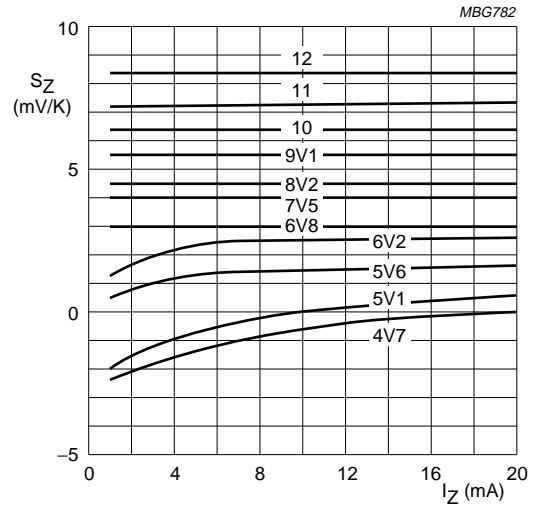
BZX55-C4V7 to C12. T_j = 25 to 150 °C.
