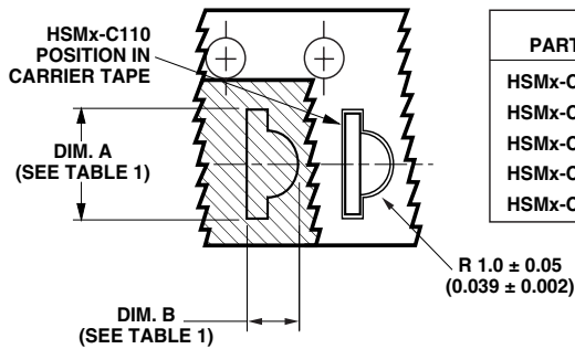
Figure 15. Tape dimensions.
