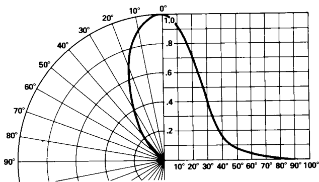
Figure 4. Relative luminous intensity vs. angular displacement for T-13 1/4 lamp.
