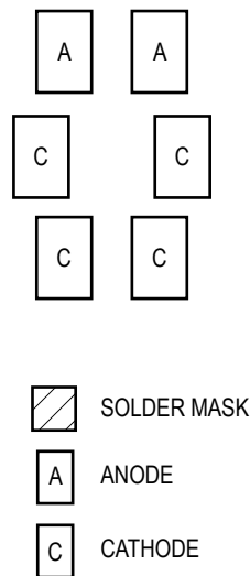
Figure 12. Recommended Soldering Pad Pattern
