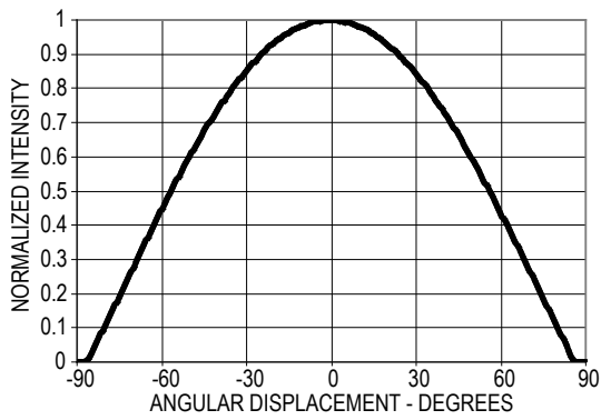
Figure 9. Radiation Pattern
