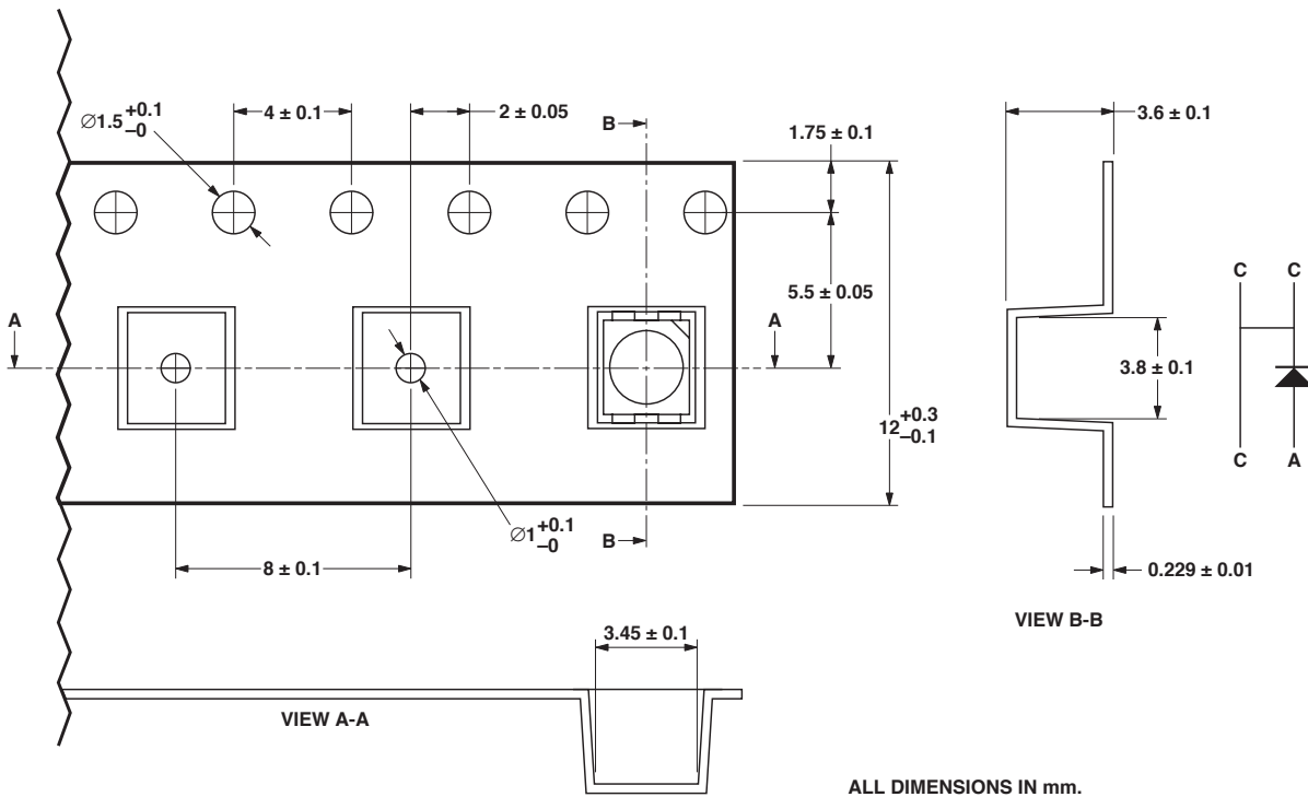
Figure 12. Tape dimensions
