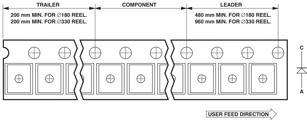
Figure 11. Tape leader and trailer dimensions
