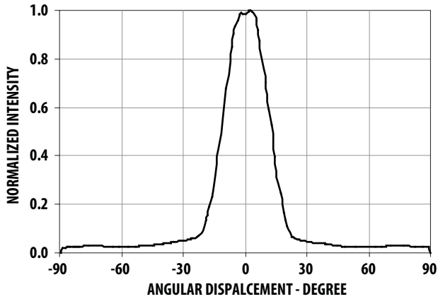
Figure 7. Radiation Pattern for 23°
