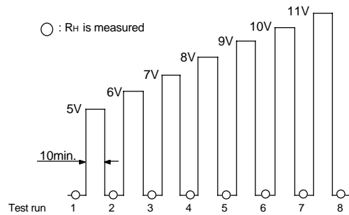
Fig. 21 - Test procedure for heater durability
