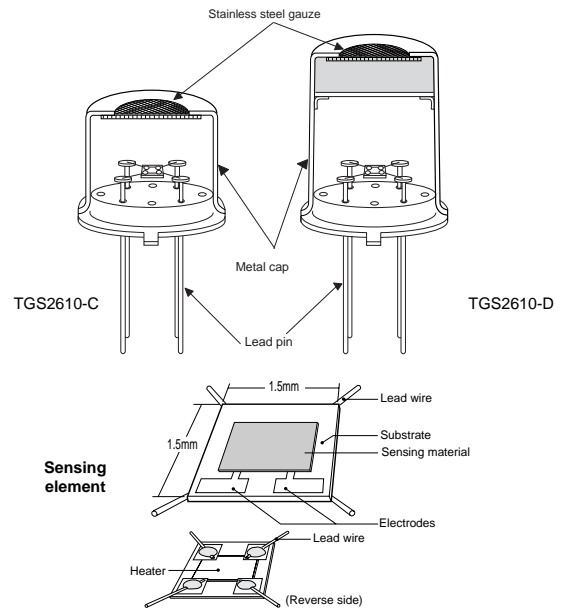
Fig. 1 - Sensor structure
