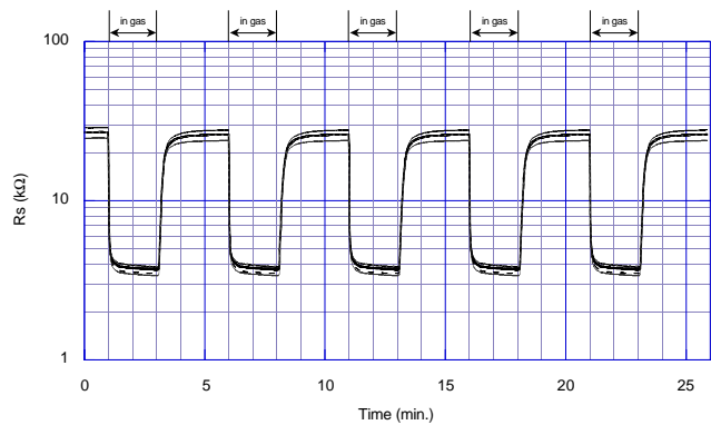
Fig. 11 - Repeatability
