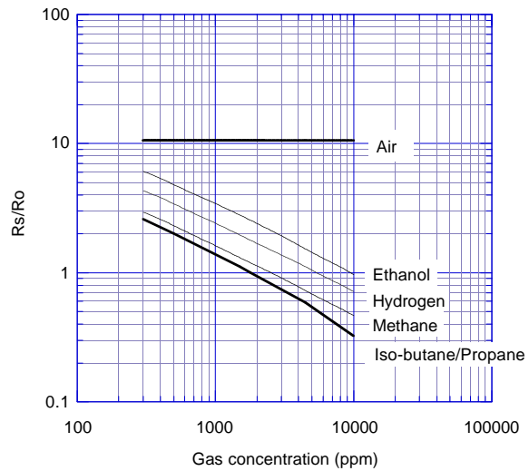
Fig. 4a - TGS2610-C00 sensitivity to various gases ( R_s/R_o )
