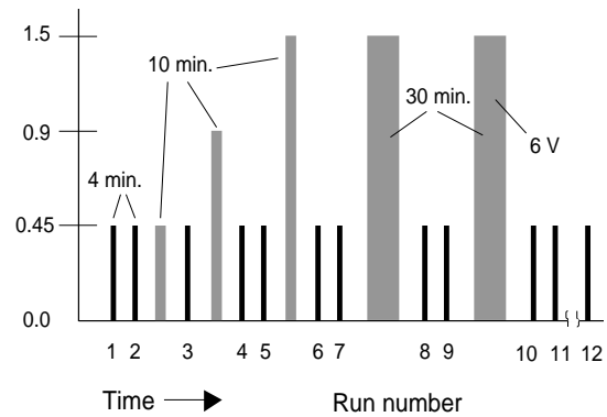
Fig. 15 - Test procedure for gas exposure
