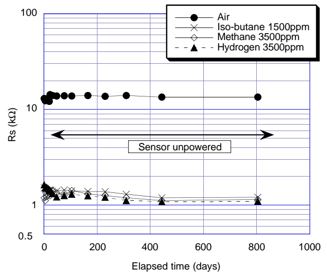
Fig. 14 - Influence of unenergizing on TGS2610-C
