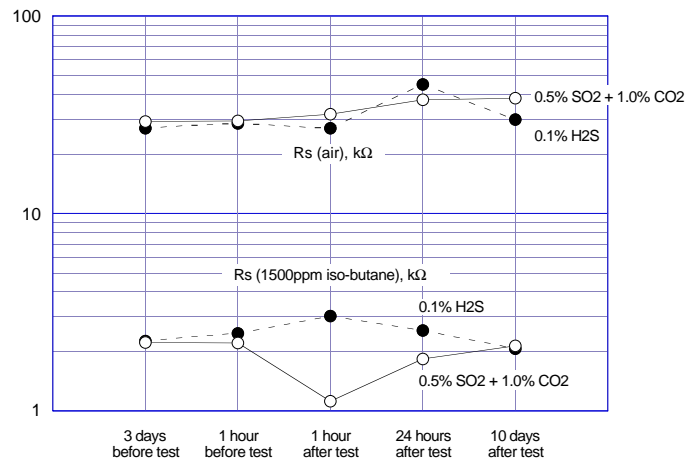
Fig. 19 - Corrosion test of TGS2610-C
