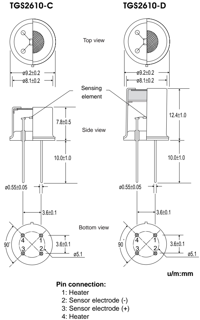
Fig. 3 - Sensor dimensions
