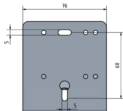
Mounting site rain alarm unit
