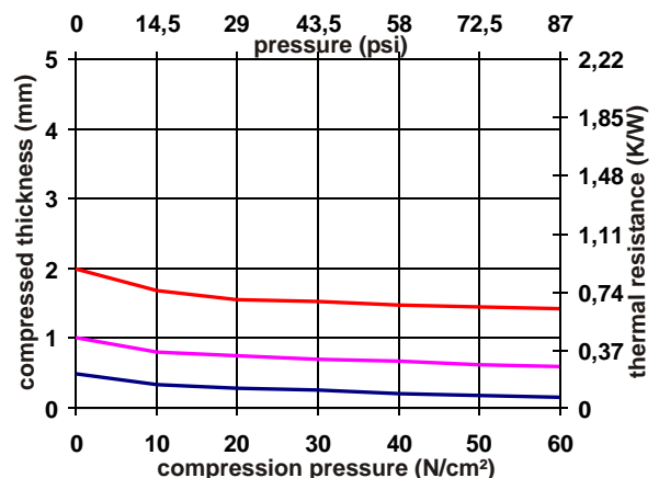
Compressibilities of Softtherm® 86/500
