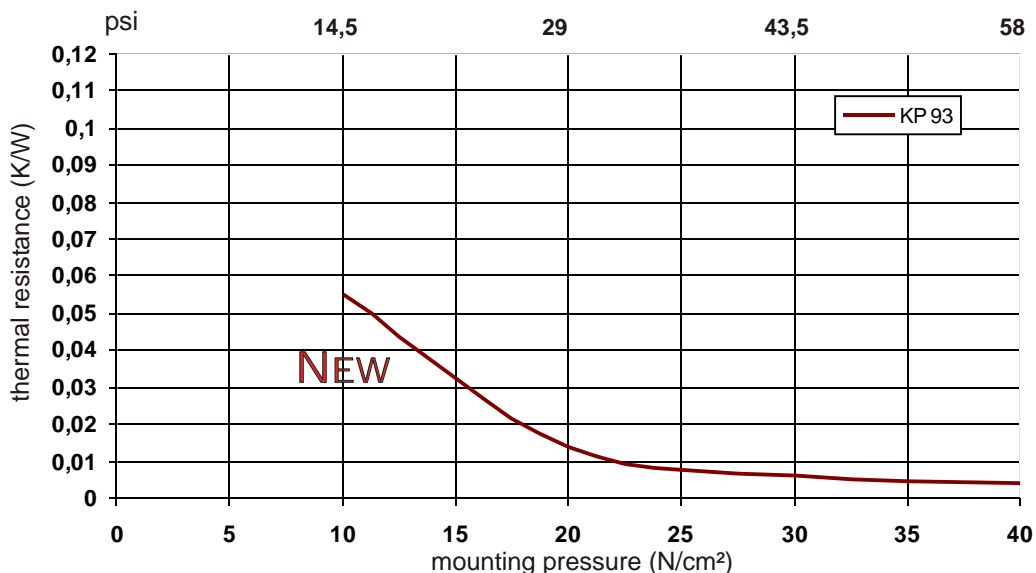
Comparison of the thermal resistance of KP 12 silicone free in dependence on the contact pressure
