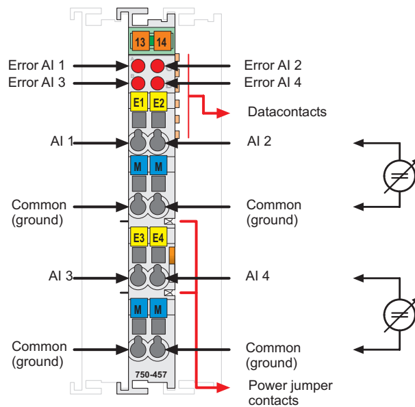
Fig. 2.1.1-1: 4-Channel Analog Input Module 750-457
