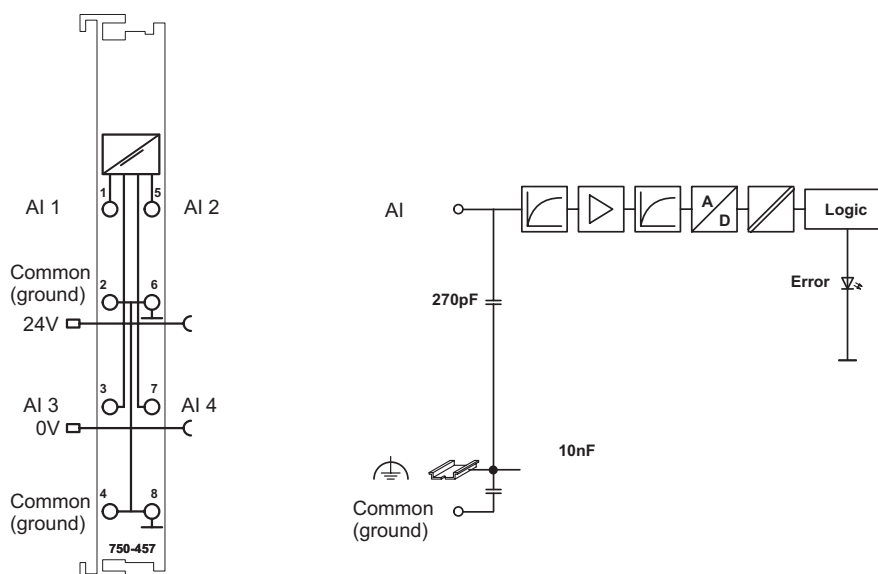
Fig. 2.1.1-3: 4-Channel Analog Input Module 750-457
