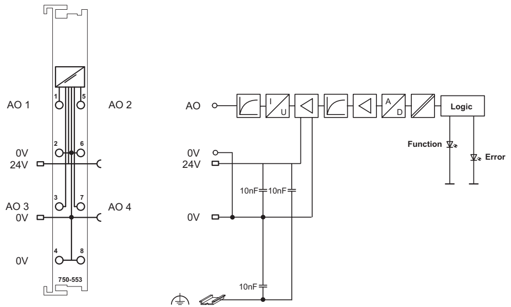
Fig. 2.1.1-3: Schematic diagram
