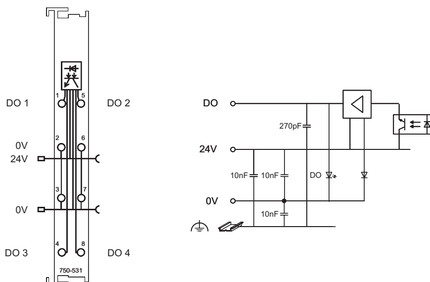
Fig. 2.1.1-3: 4-Channel Digital Output Module 750-531
