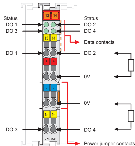
Fig. 2.1.1-1: 4-Channel Digital Output Module 750-531
