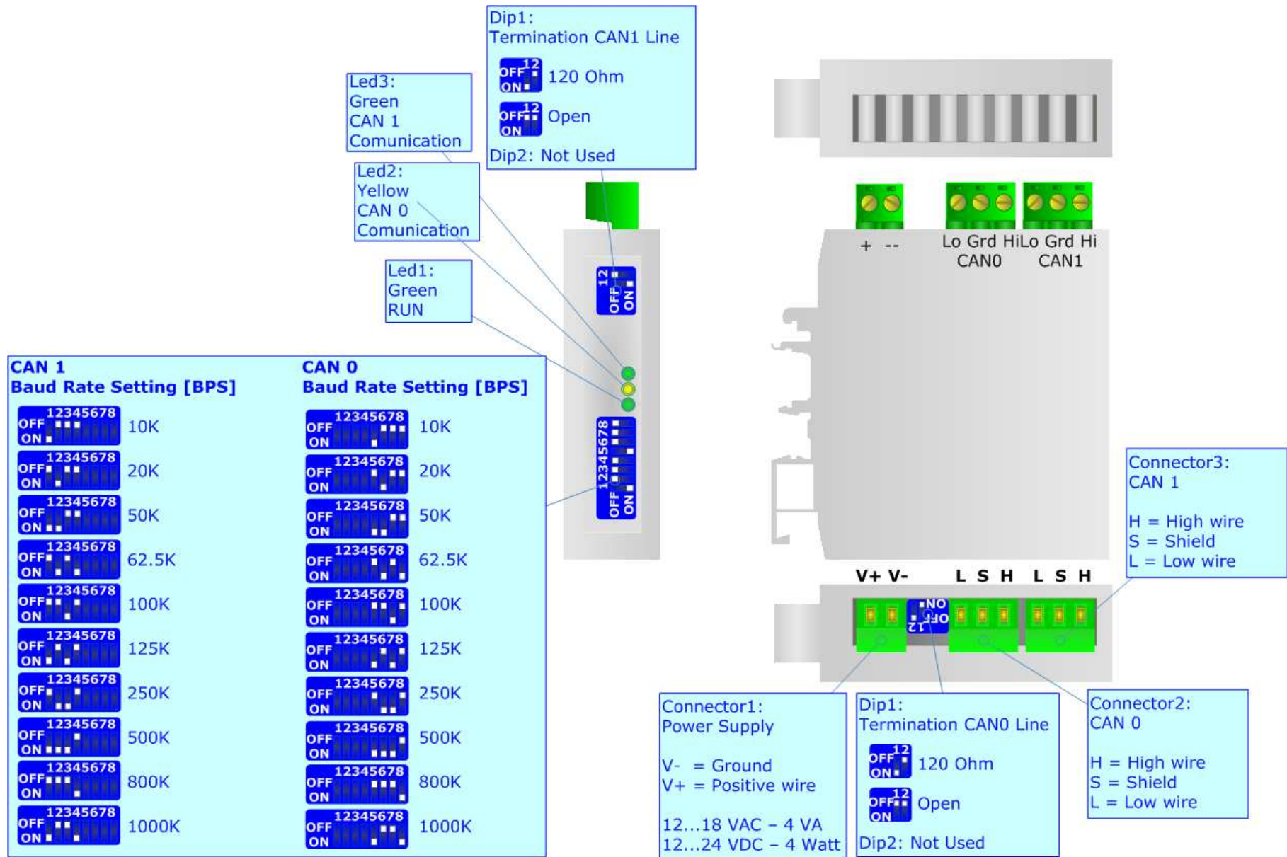
Figure 4: Connection scheme for HD67117R
