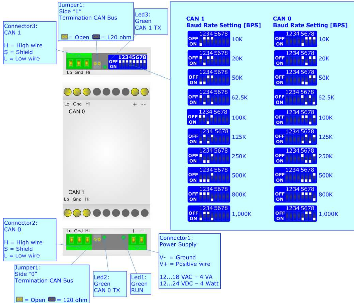
Figure 2: Connection scheme for HD67117M
