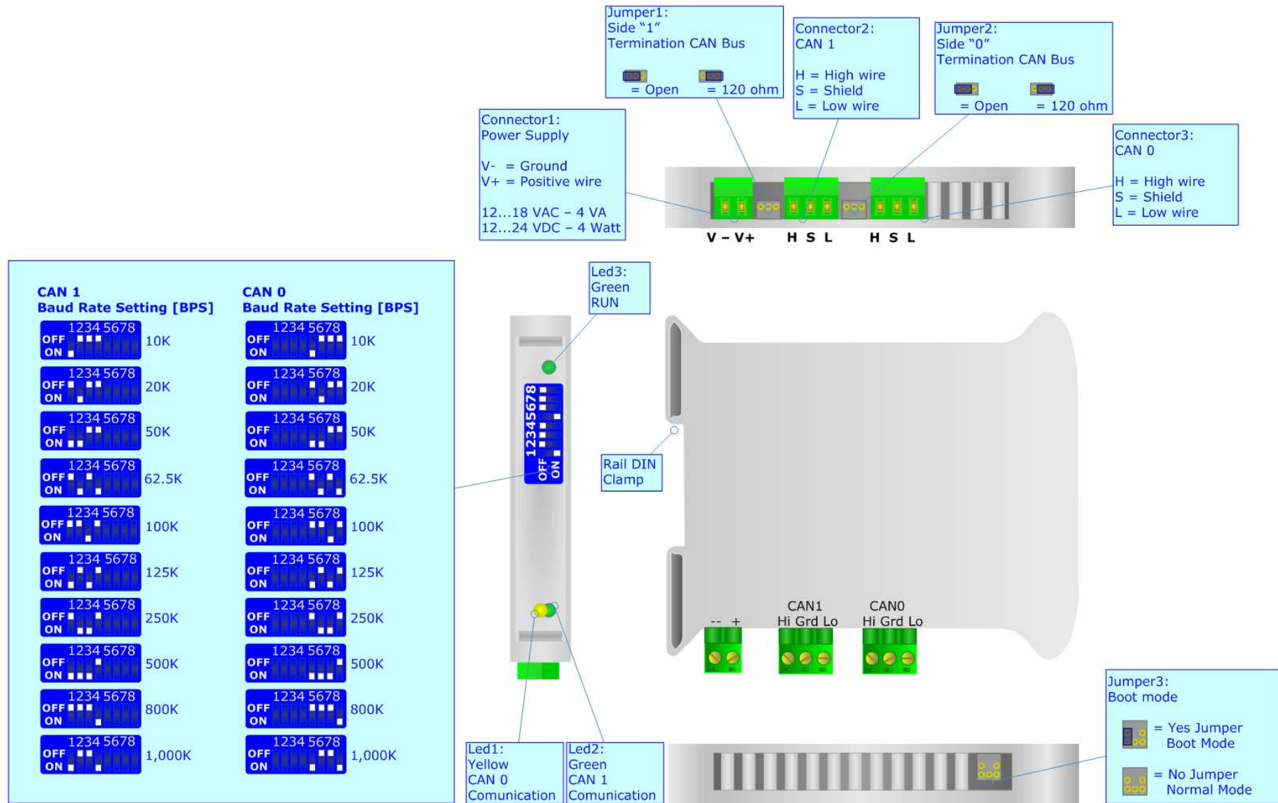
Figure 1: Connection scheme for HD67117
