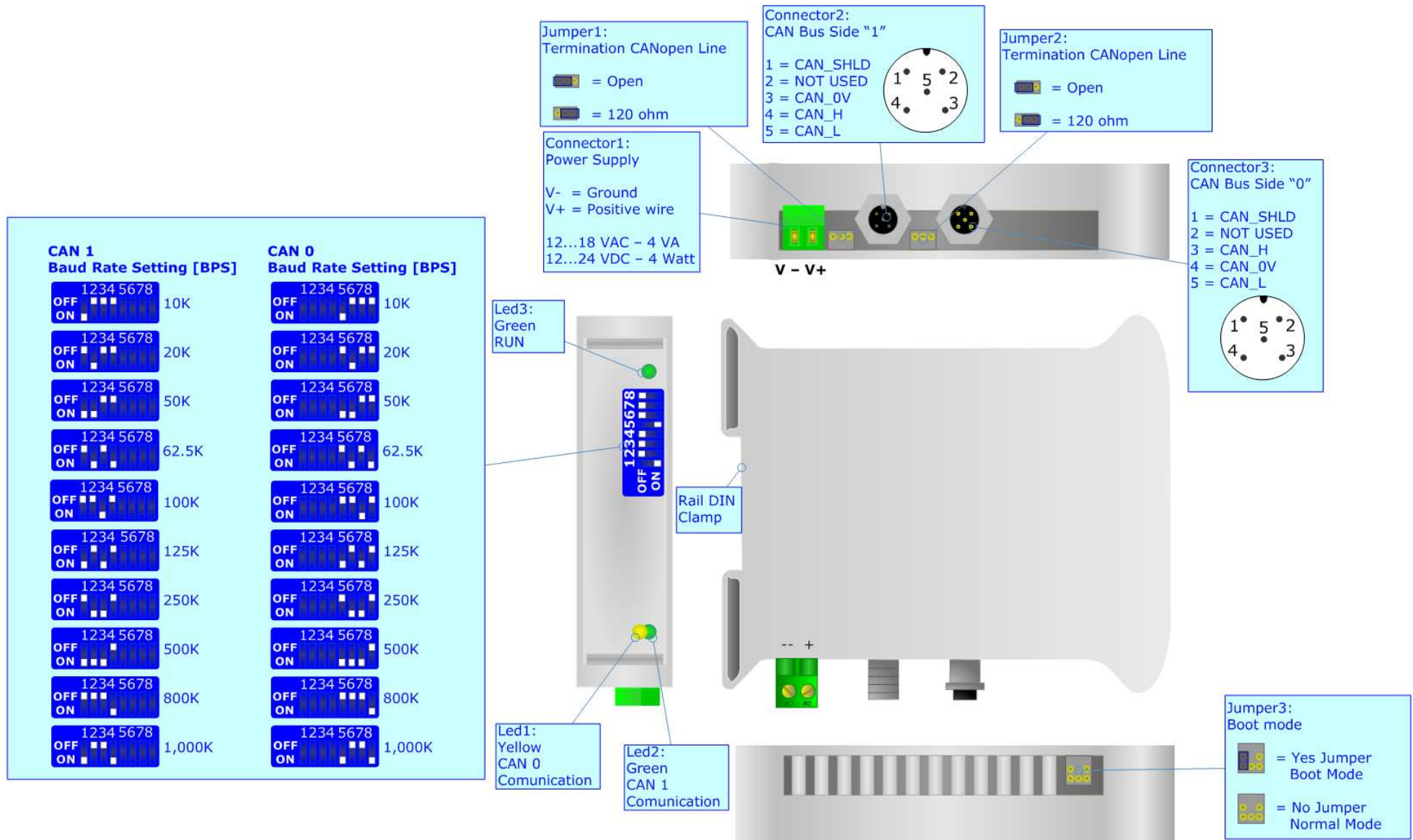
Figure 3: Connection scheme for HD67117-M12
