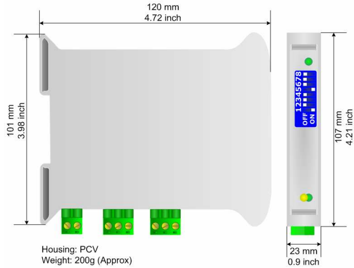
Figure 4: Mechanical dimensions scheme for HD67181
