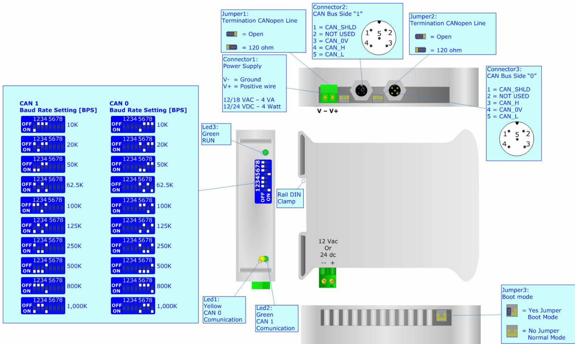
Figure 3: Connection scheme for HD67181-M12
