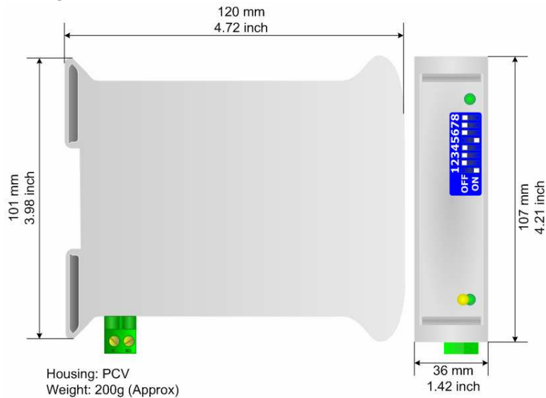
Figure 6: Mechanical dimensions scheme for HD67181-M12
