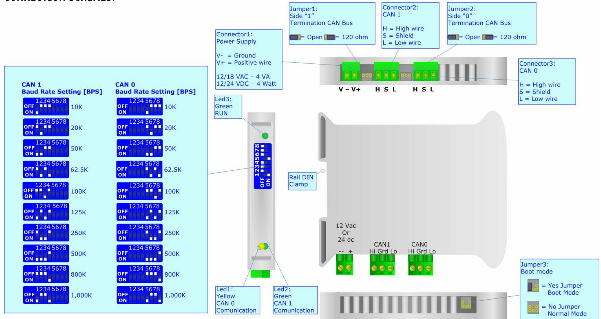
Figure 1: Connection scheme for HD67181
