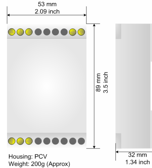
Figure 5: Mechanical dimensions scheme for HD67181M
