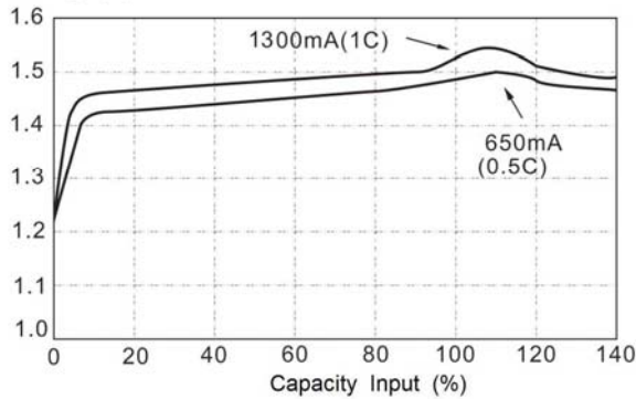
Low Rate Discharge Voltage(V)
