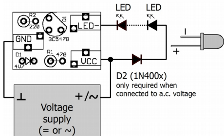
Fig. 2 Connections diagram
