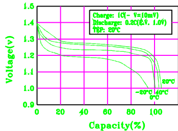
DISCHARGE CHARACTERISTICS AT DIFFERENT TEMPERATURE
