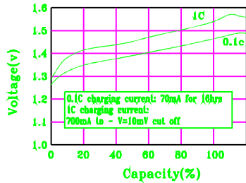
CHARGE CHARACTERISTICS
