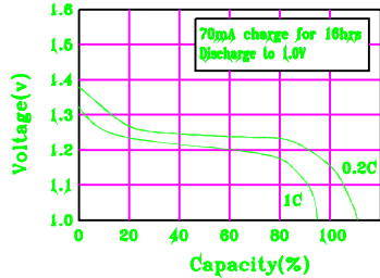
DISCHARGE CHARACTERISTICS
