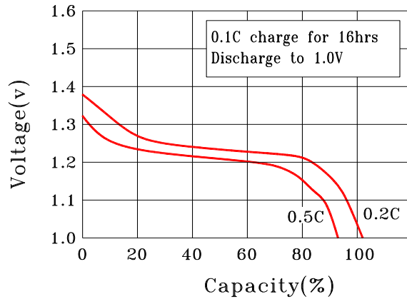
DISCHARGE CHARACTERISTICS
