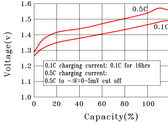
CHARGE CHARACTERISTICS
