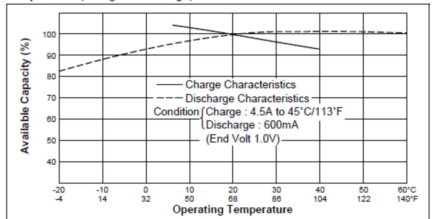
Temperature (Charge & Discharge)
