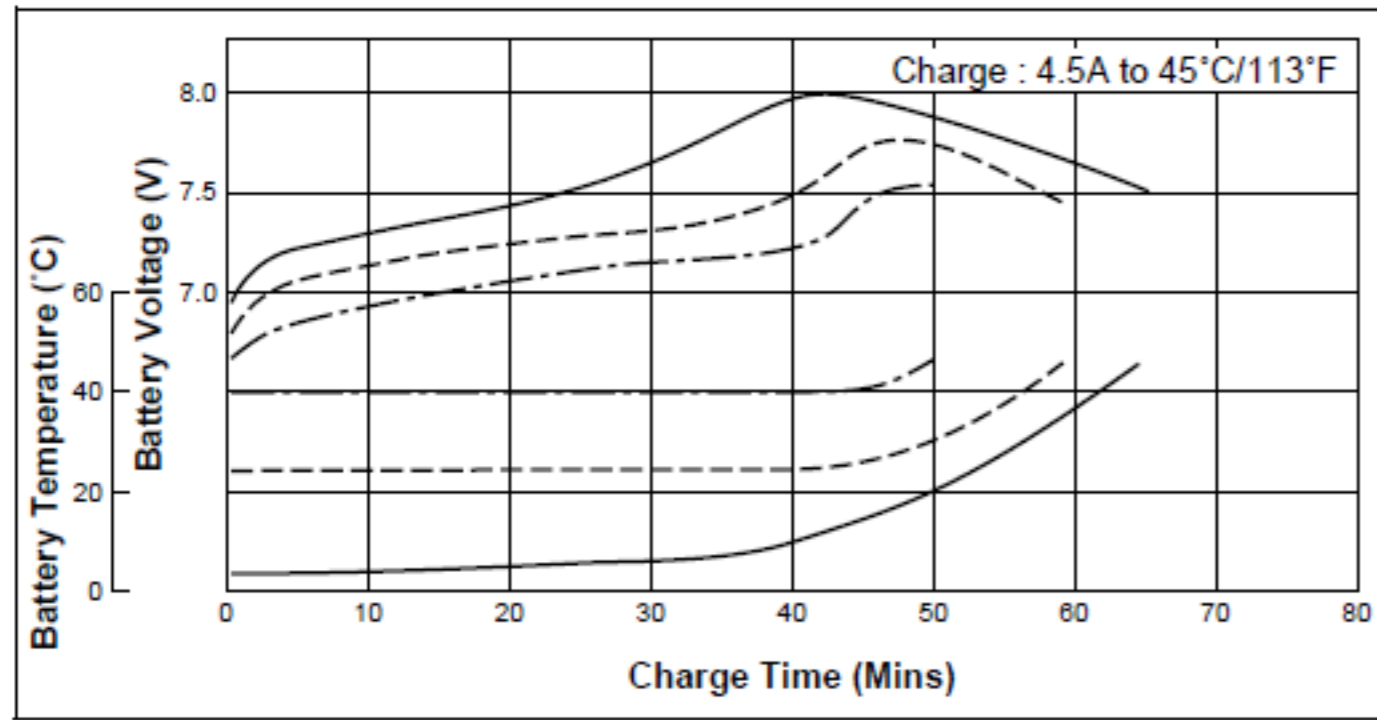
Charge (5 cells pack)
