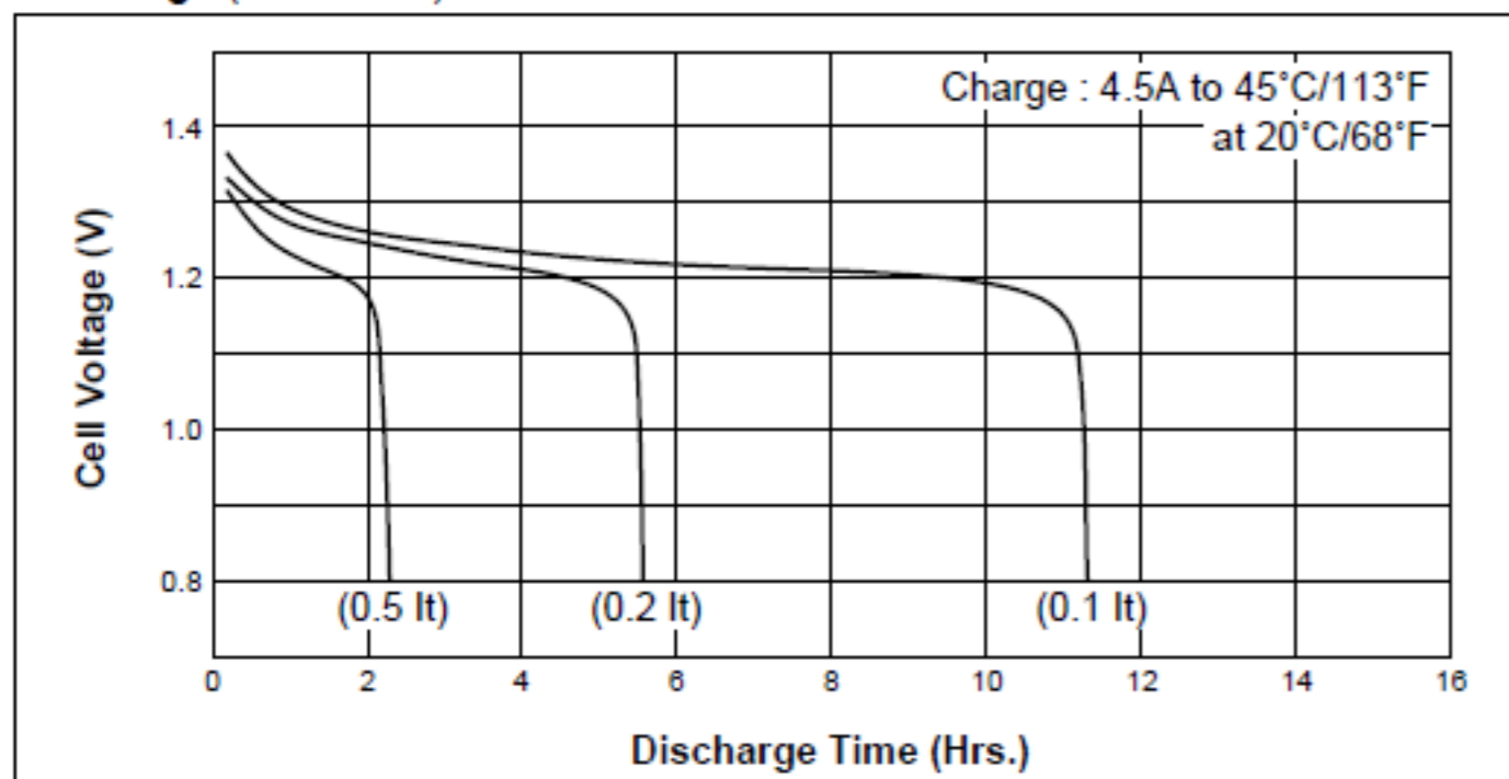
Discharge (at low rate)
