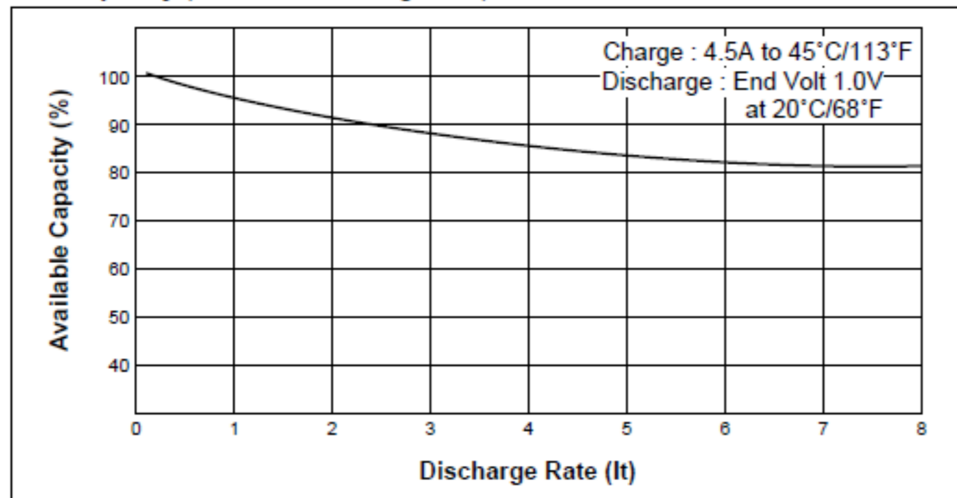
Cell Capacity (at various discharge rate)
