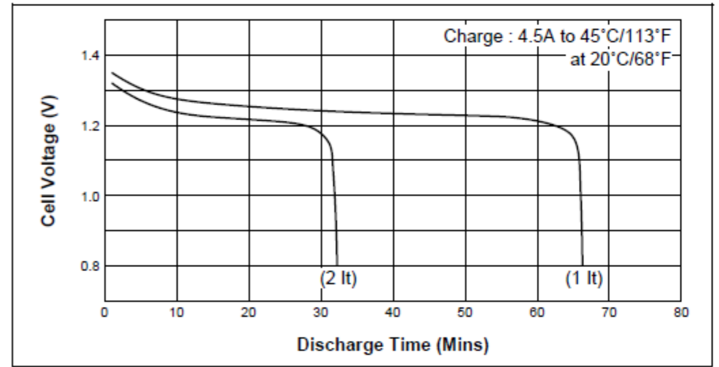
Discharge (at high rate)
