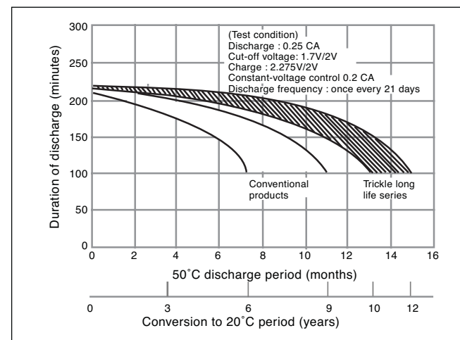
Trickle life characteristics at 50°C
