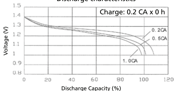
Discharge characteristics
