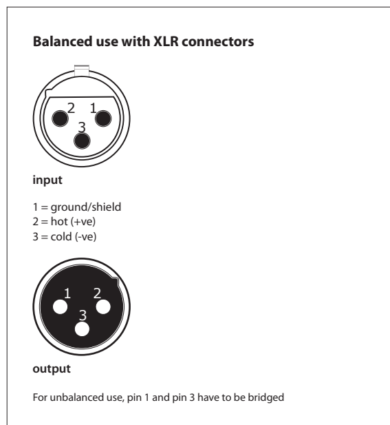
Fig. 4.1: XLR connectors
