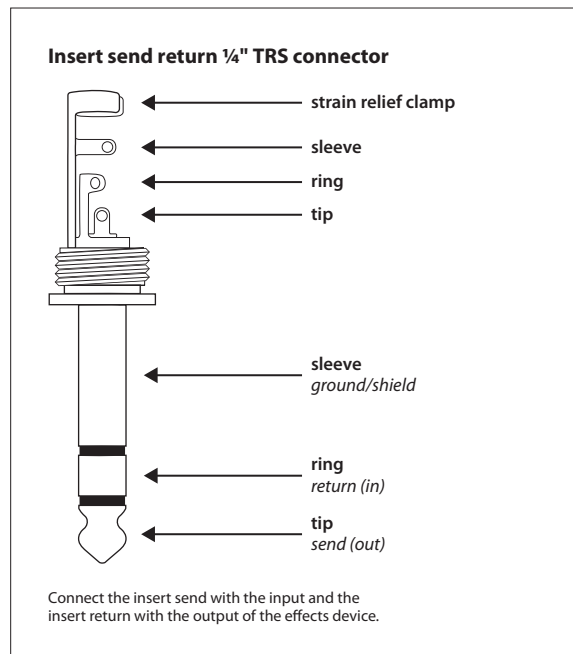
Fig. 4.4: ¼" TRS connector for insert send/return applications
