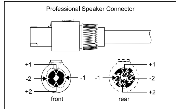
Fig. 6.1: Professional speaker connector
