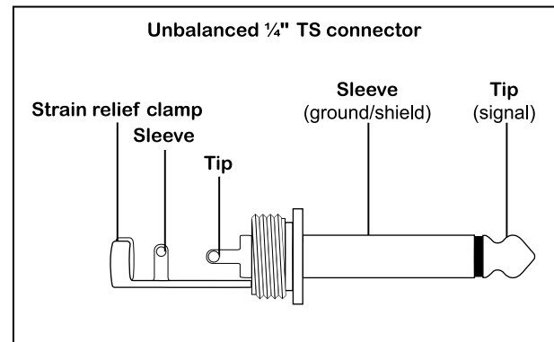
Fig. 6.2: 1/4" TS connector
