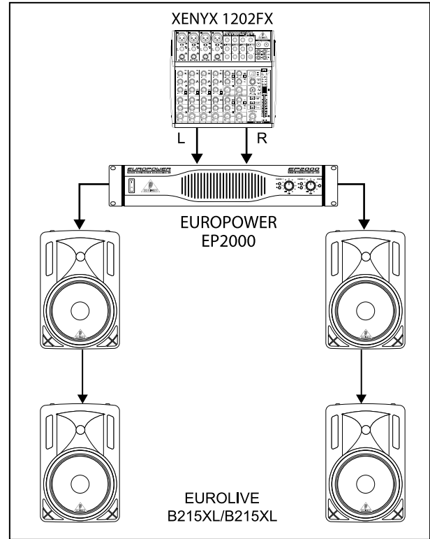
Fig. 5.2: Wiring several B212XL/B215XL loudspeakers
